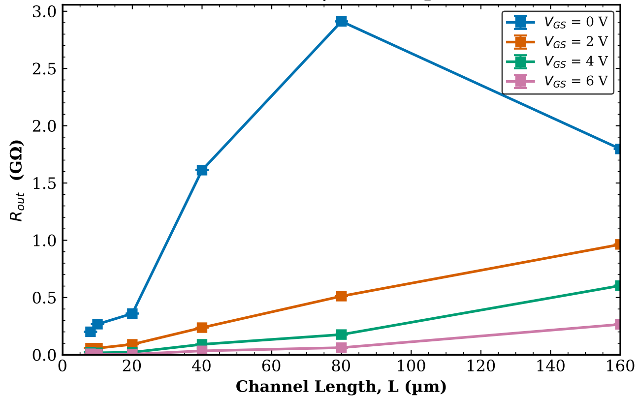
TFT1 Transistor 2 R_{out} vs L | W = 10 \mu\text{m}
